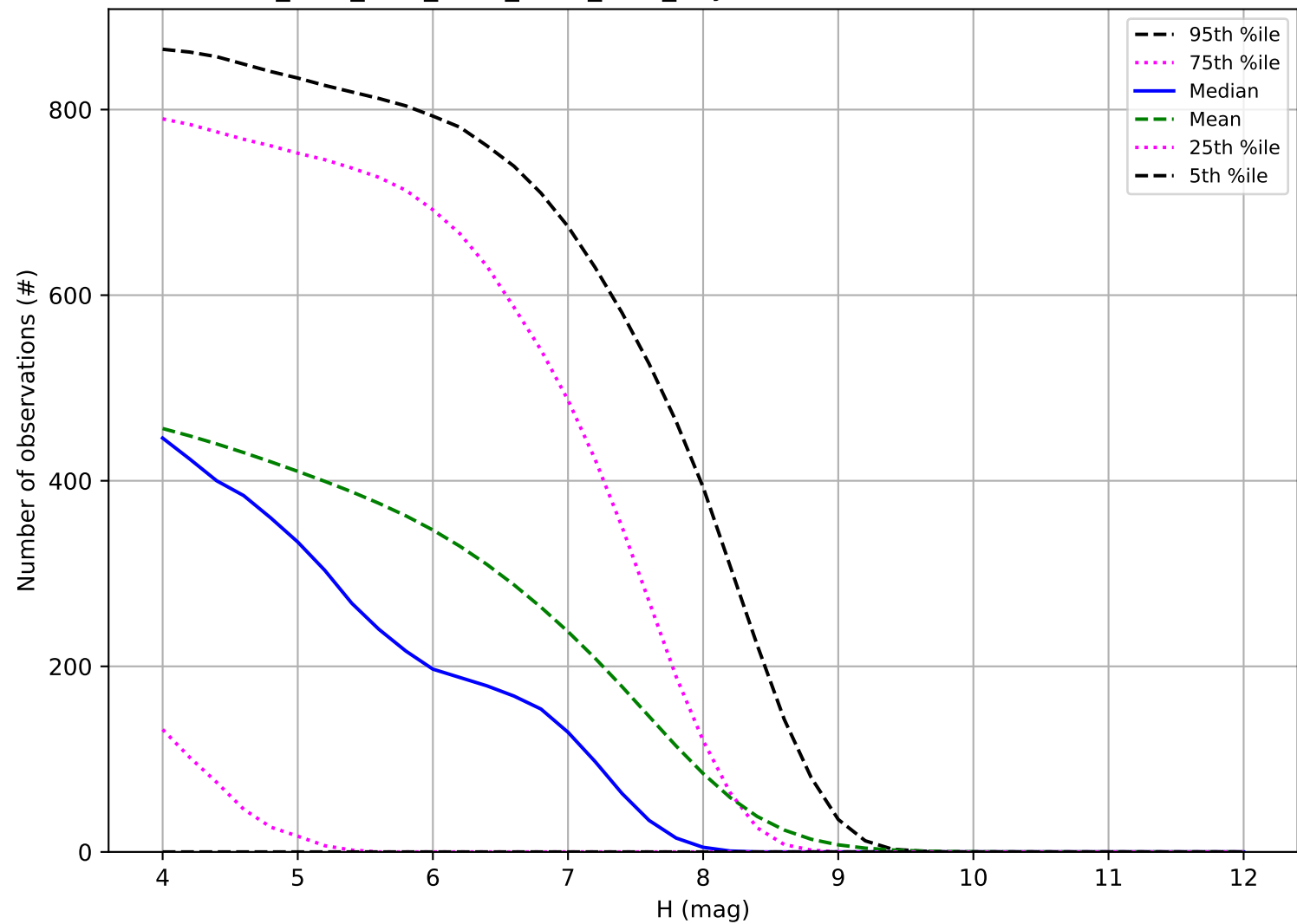
ddf_acor_sf10_lsf15_lsr10_v3.4_10yrs: Number of observations TNO
