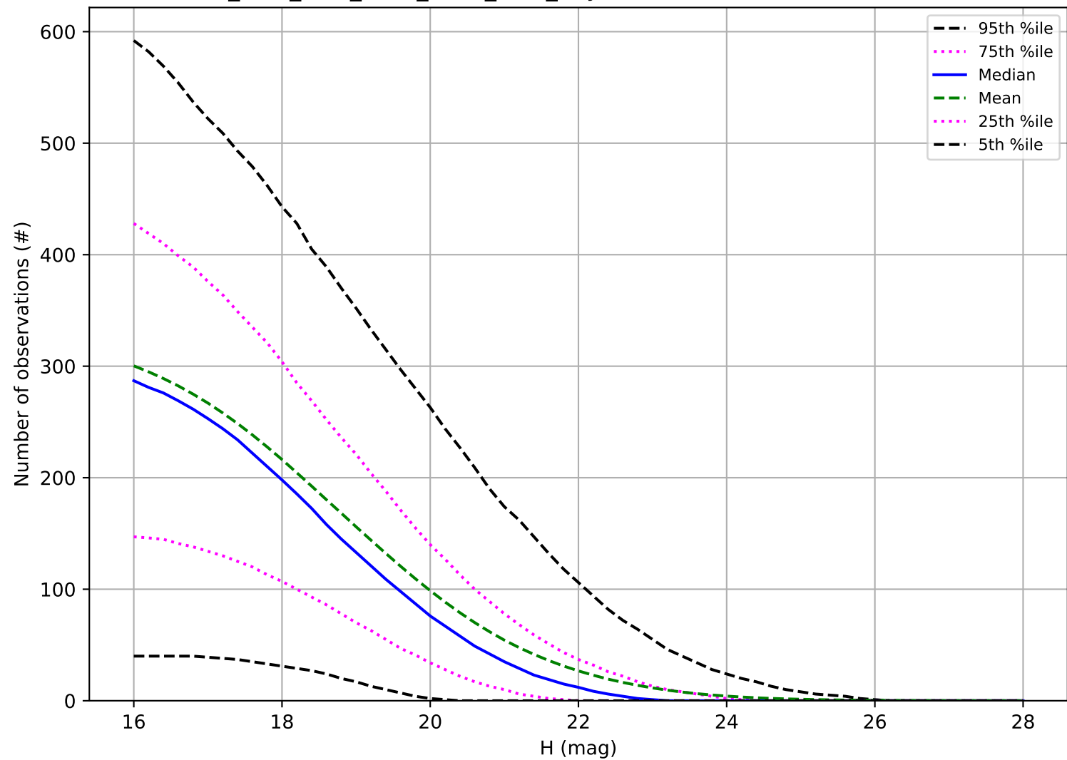
ddf_acor_sf10_lsf15_lsr10_v3.4_10yrs: Number of observations PHA
