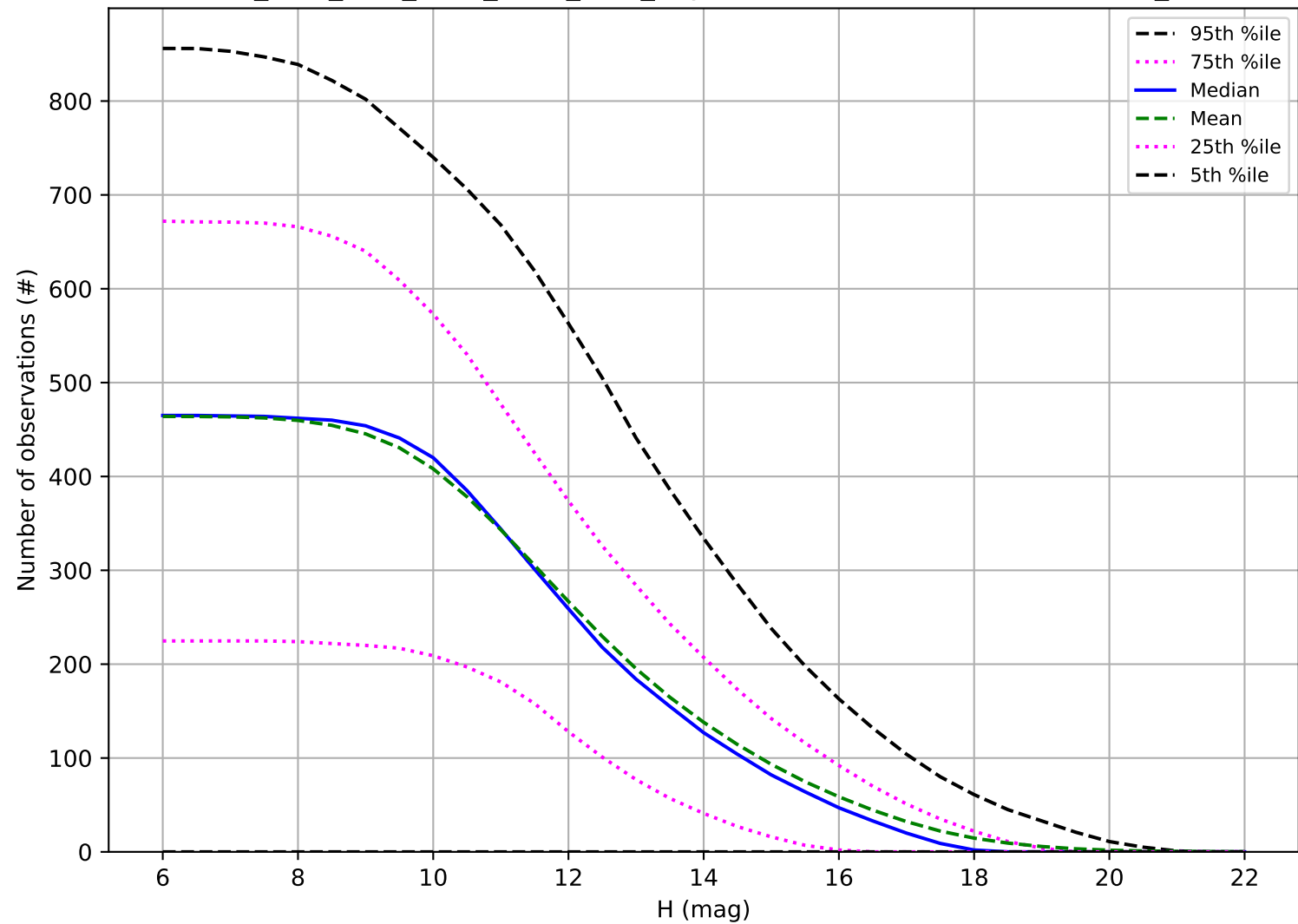
ddf_acor_sf10_lsf15_lsr10_v3.4_10yrs: Number of observations OCC_r5
