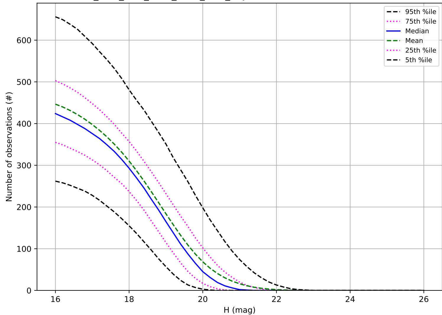
ddf_acor_sf10_lsf15_lsr10_v3.4_10yrs: Number of observations MBA
