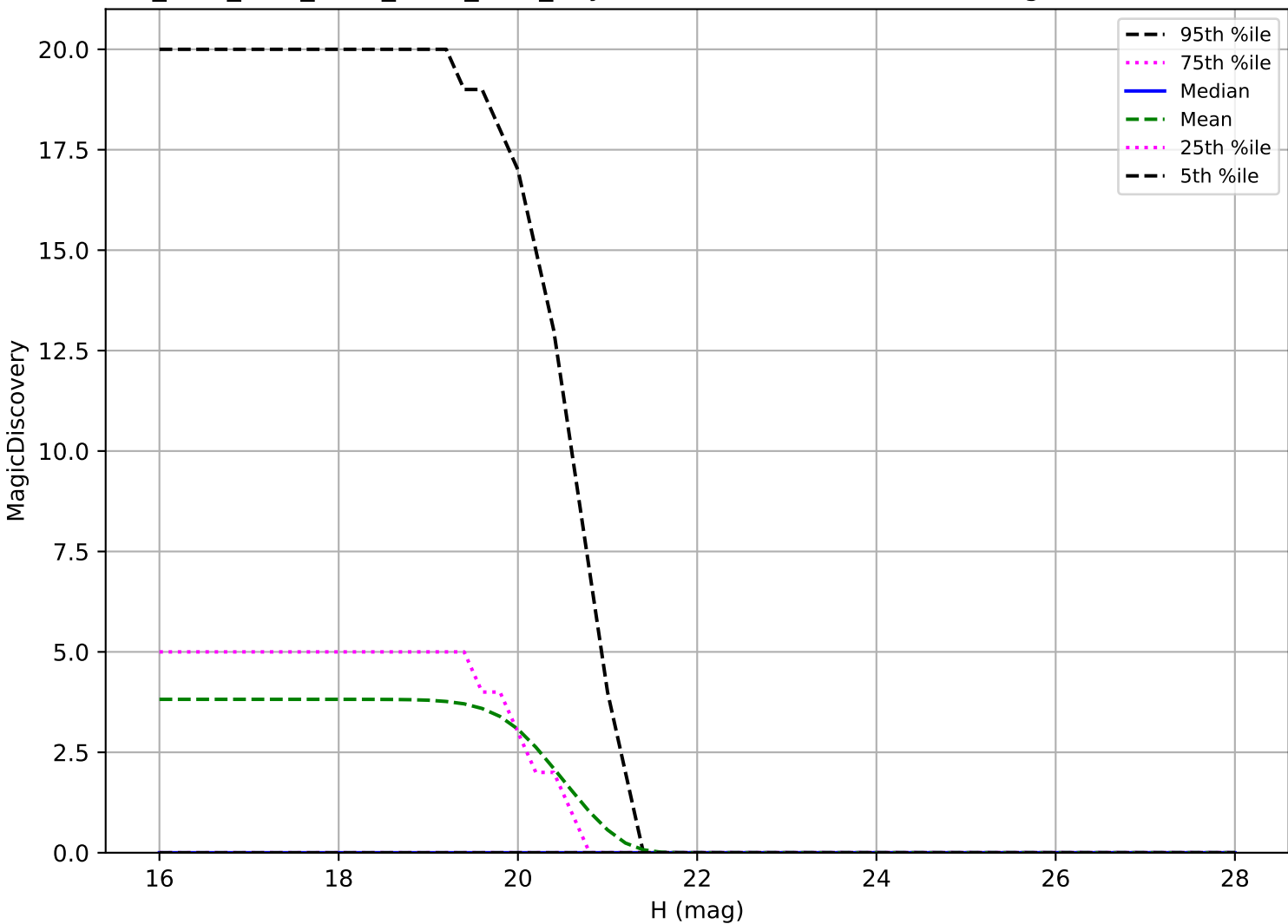
ddf_acor_sf10_lsf15_lsr10_v3.4_10yrs: Vatra 6 detections in 60 nights detection loss
