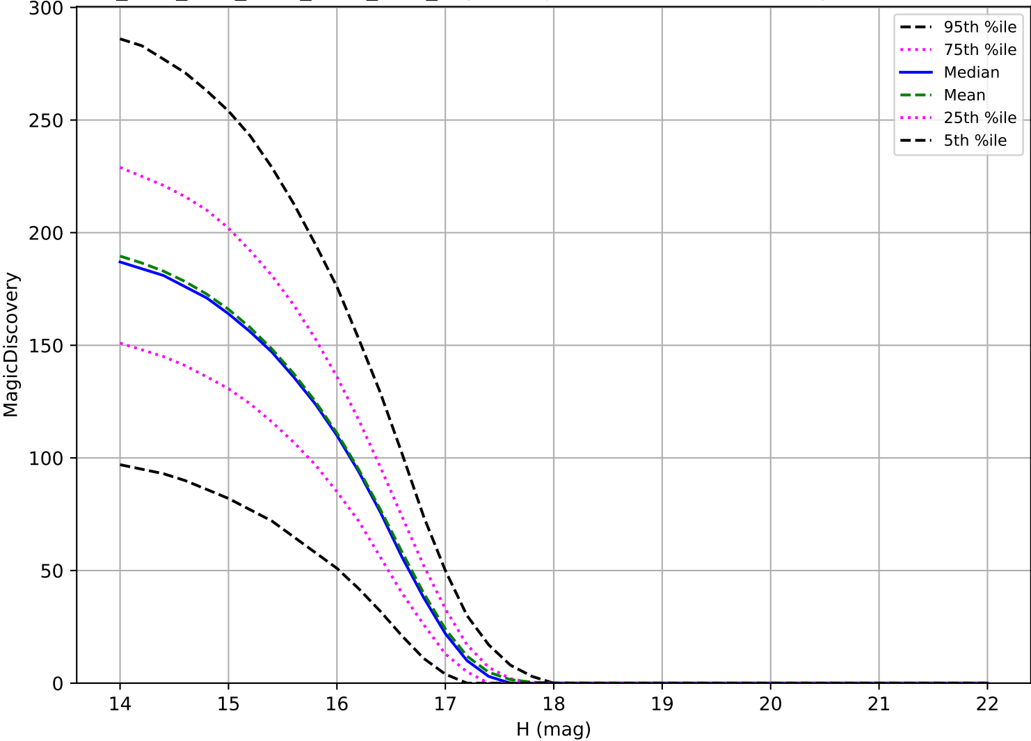
ddf_acor_sf10_lsf15_lsr10_v3.4_10yrs: Trojan 6 detections in 60 nights detection loss
