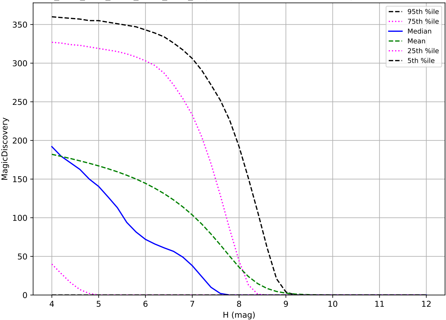
ddf_acor_sf10_lsf15_lsr10_v3.4_10yrs: TNO 6 detections in 60 nights detection loss
