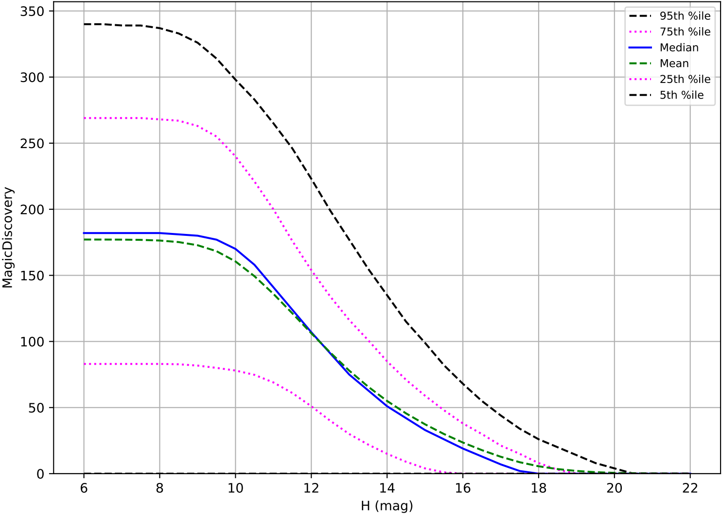
ddf_acor_sf10_lsf15_lsr10_v3.4_10yrs: OCC_r5 6 detections in 60 nights detection loss
