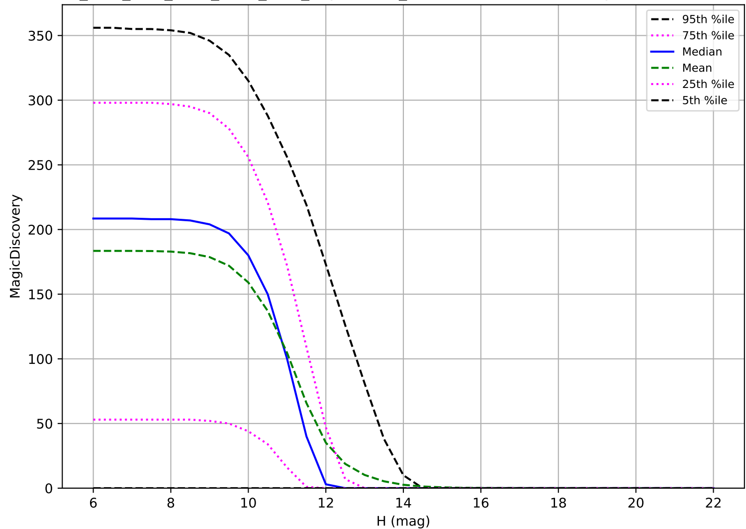
ddf_acor_sf10_lsf15_lsr10_v3.4_10yrs: OCC_r20 6 detections in 60 nights detection loss
