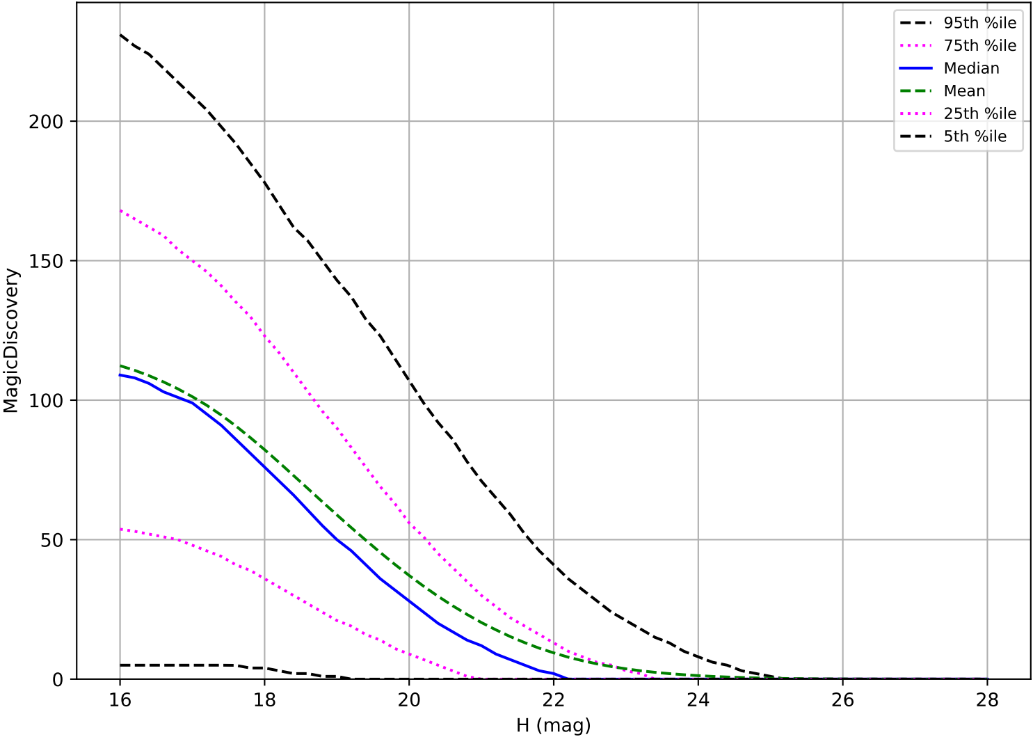
ddf_acor_sf10_lsf15_lsr10_v3.4_10yrs: NEO 6 detections in 60 nights detection loss
