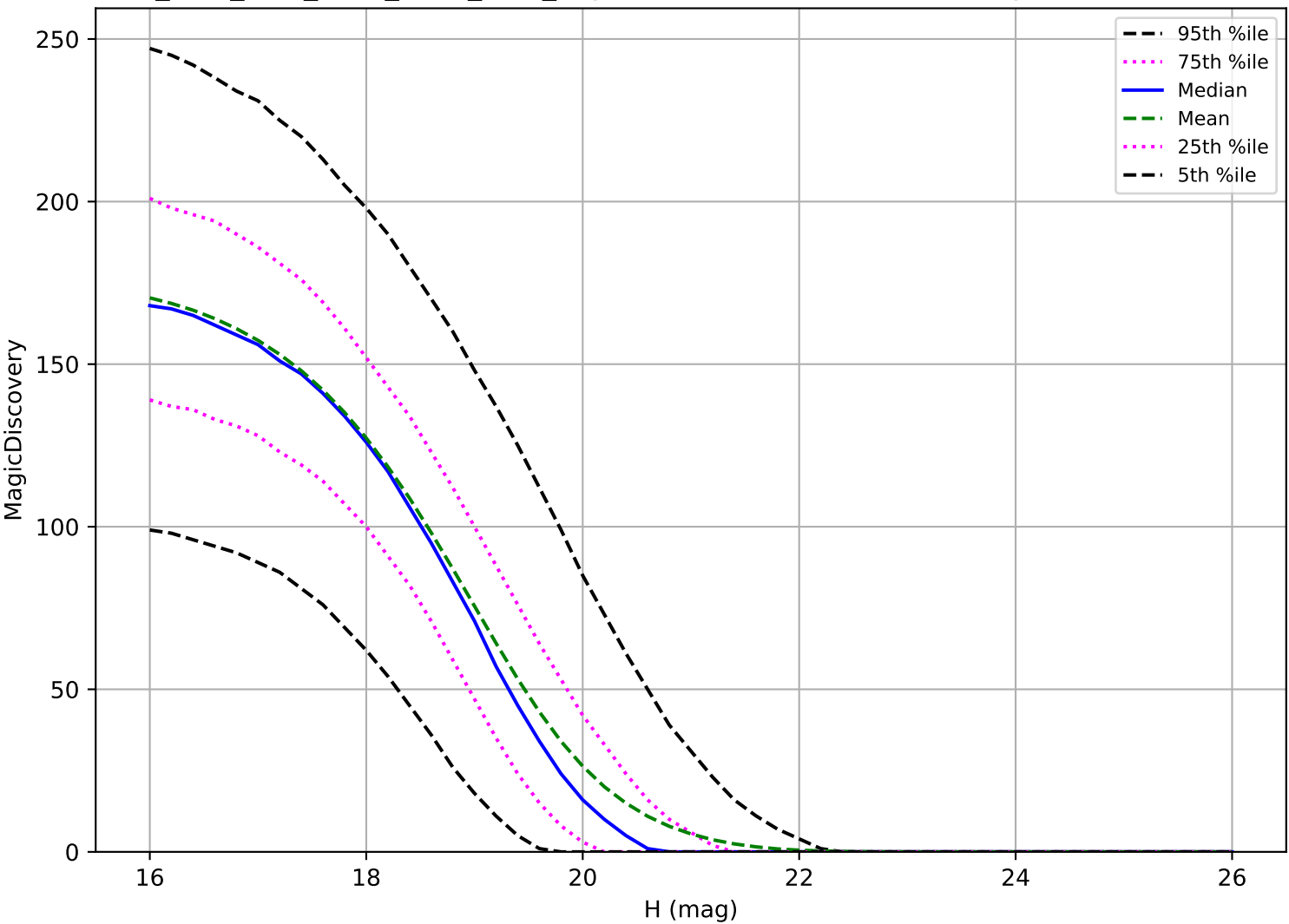
ddf_acor_sf10_lsf15_lsr10_v3.4_10yrs: MBA 6 detections in 60 nights detection loss
