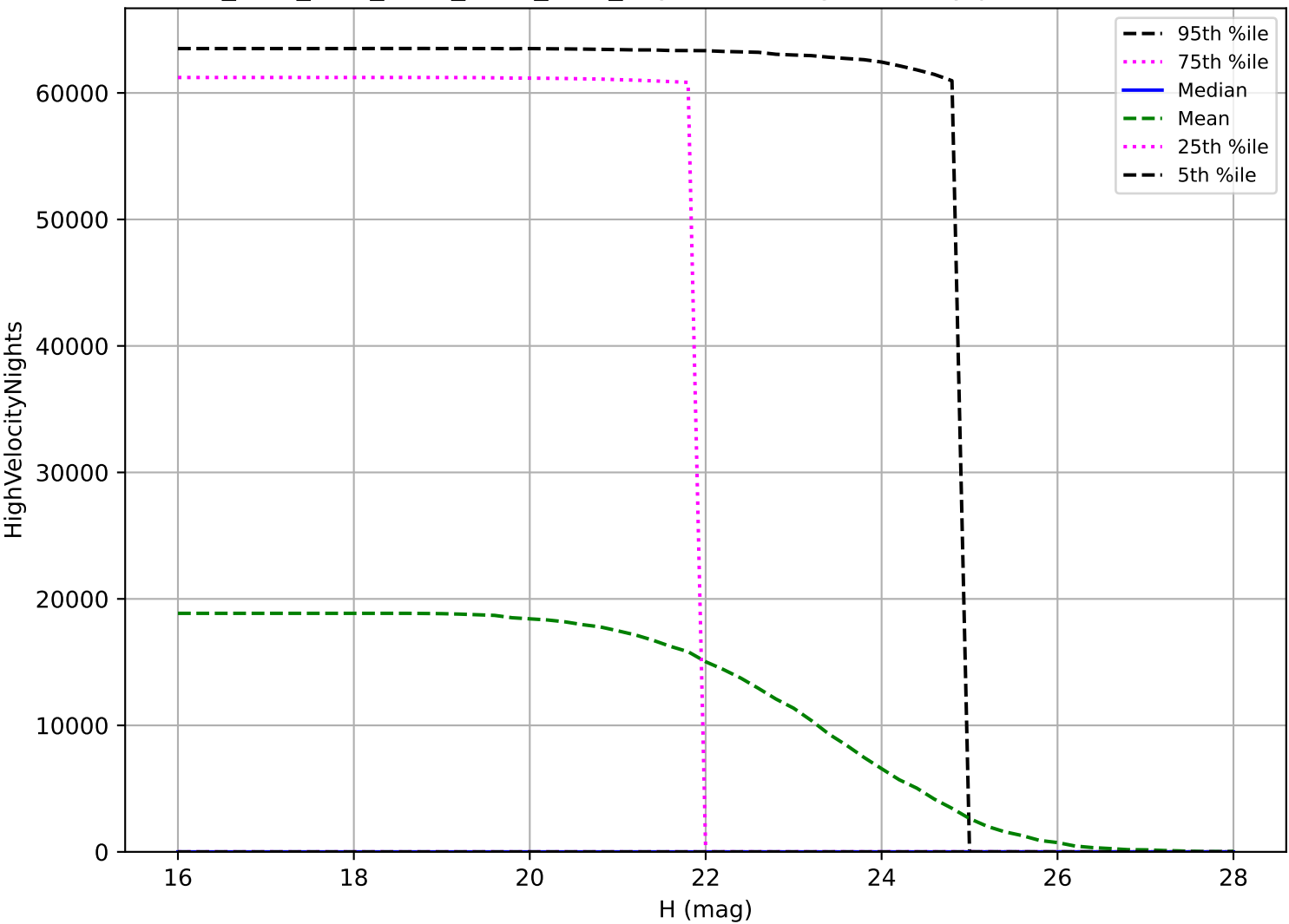
ddf_acor_sf10_lsf15_lsr10_v3.4_10yrs: NEO High velocity pair detection loss
