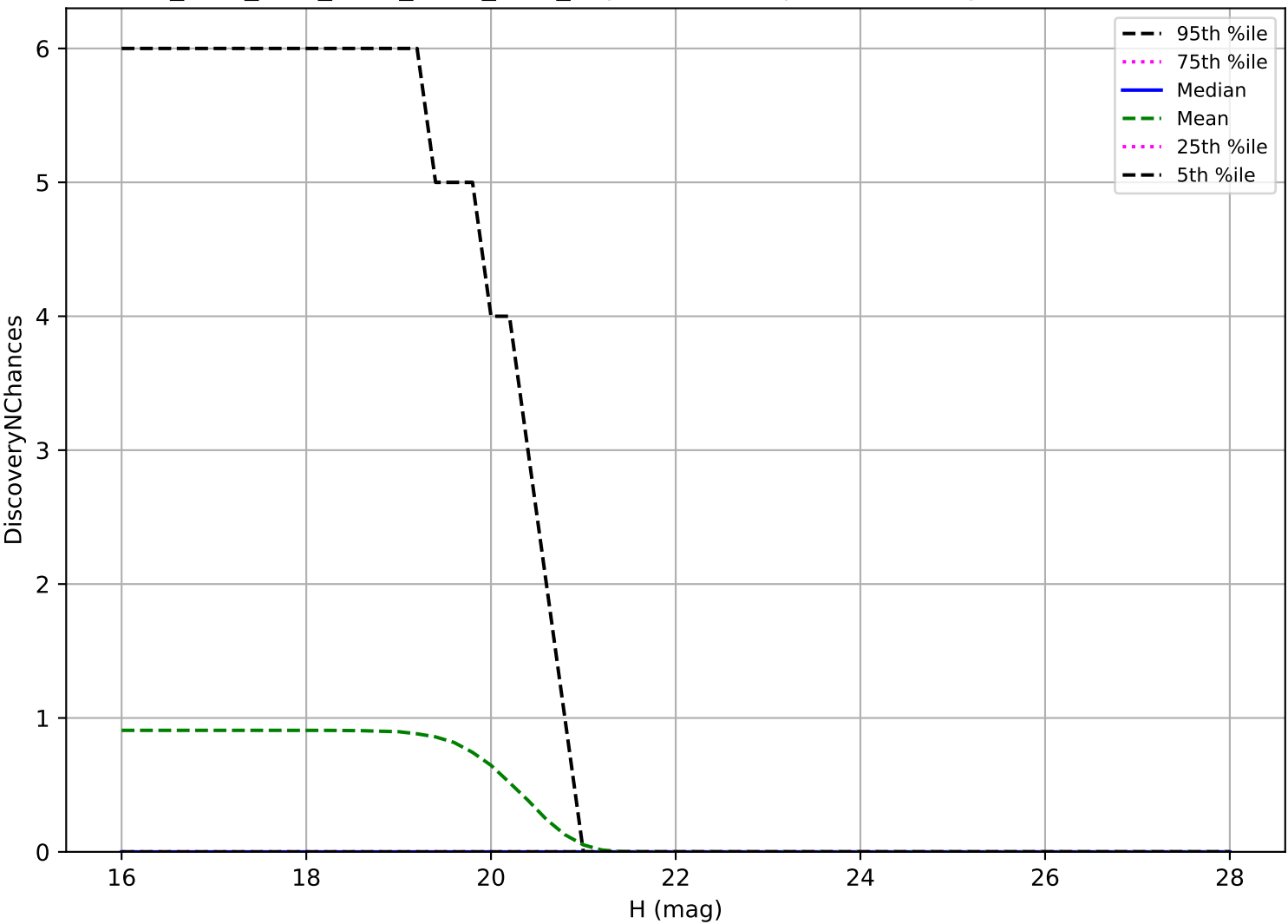
ddf_acor_sf10_lsf15_lsr10_v3.4_10yrs: Vatira 3 pairs in 15 nights detection loss
