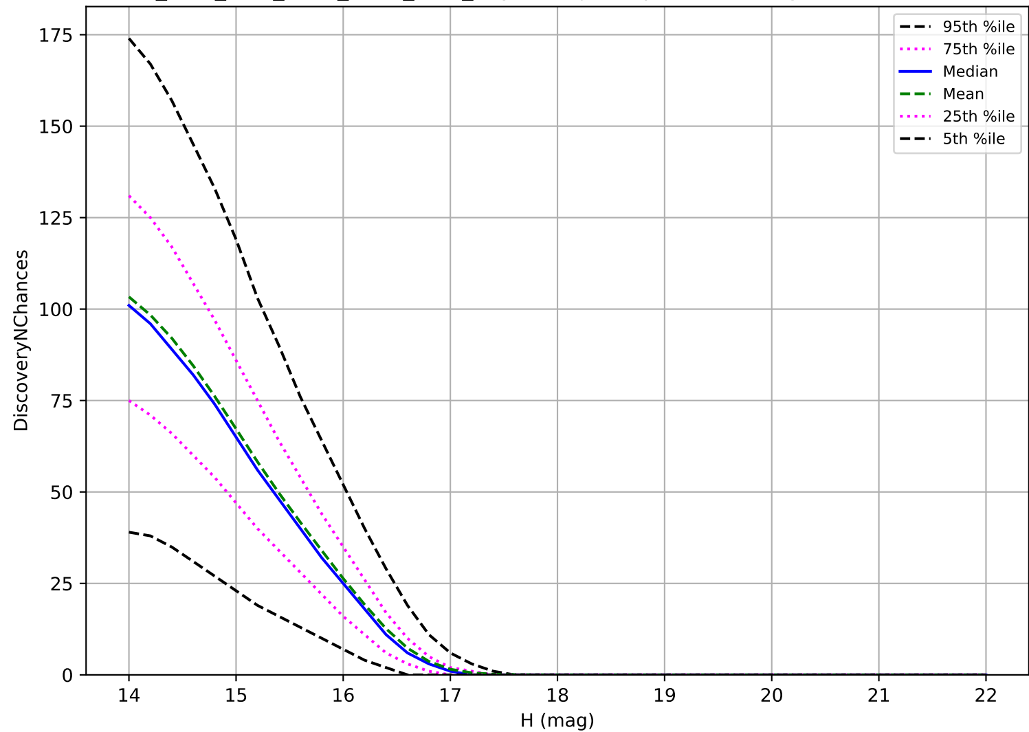
ddf_acor_sf10_lsf15_lsr10_v3.4_10yrs: Trojan 3 pairs in 15 nights detection loss
