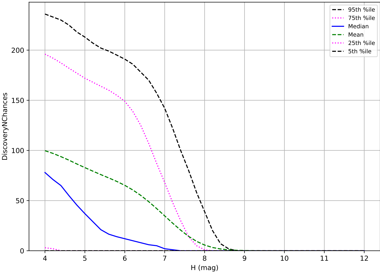
ddf_acor_sf10_lsf15_lsr10_v3.4_10yrs: TNO 3 pairs in 15 nights detection loss
