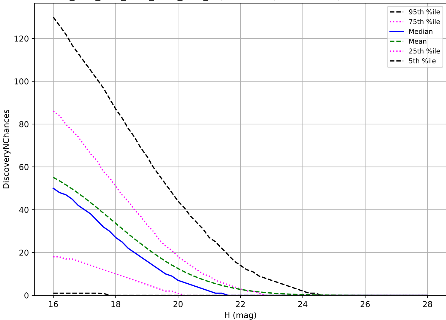
ddf_acor_sf10_lsf15_lsr10_v3.4_10yrs: PHA 3 pairs in 15 nights detection loss
