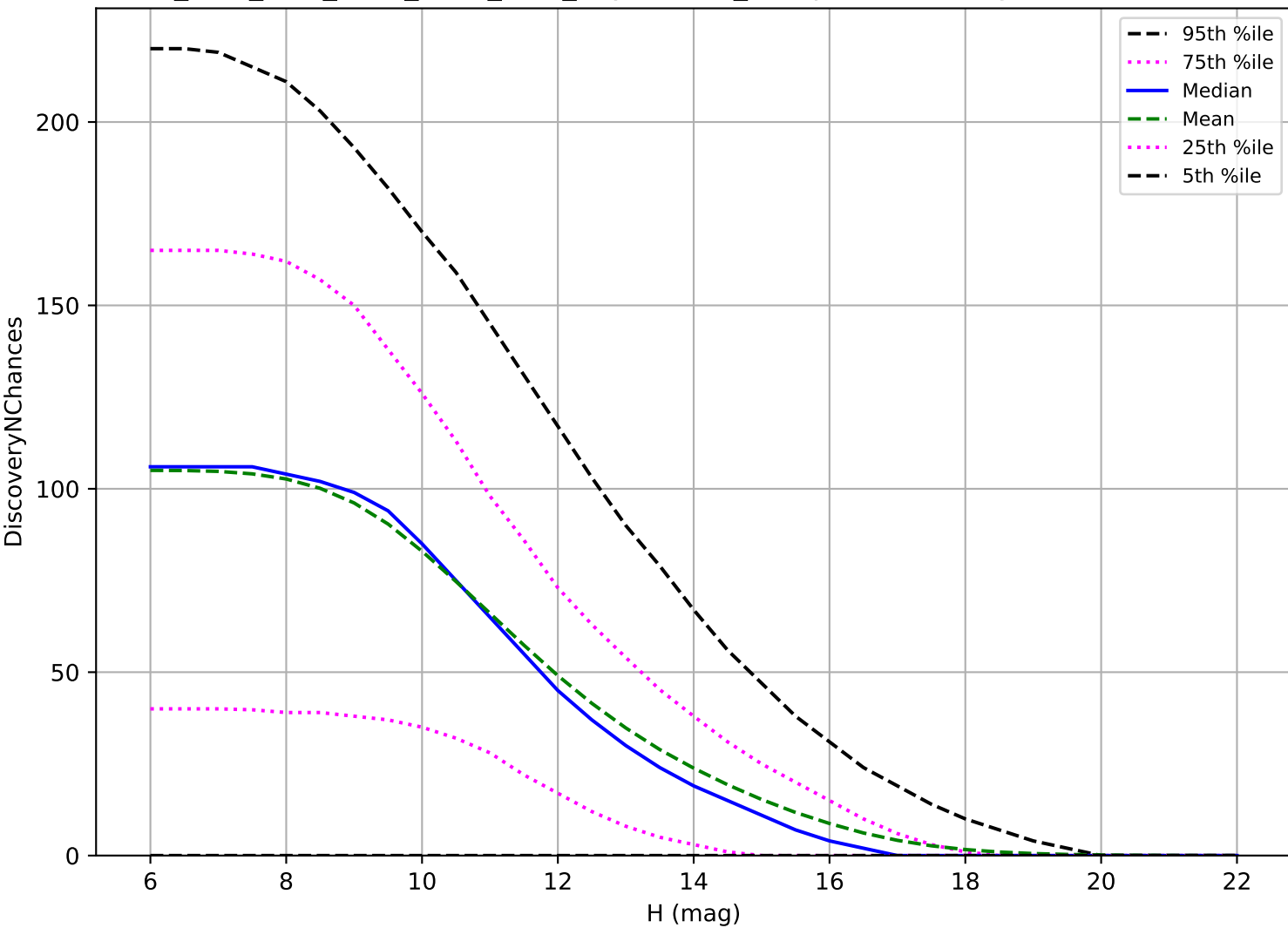
ddf_acor_sf10_lsf15_lsr10_v3.4_10yrs: OCC_r5 3 pairs in 15 nights detection loss
