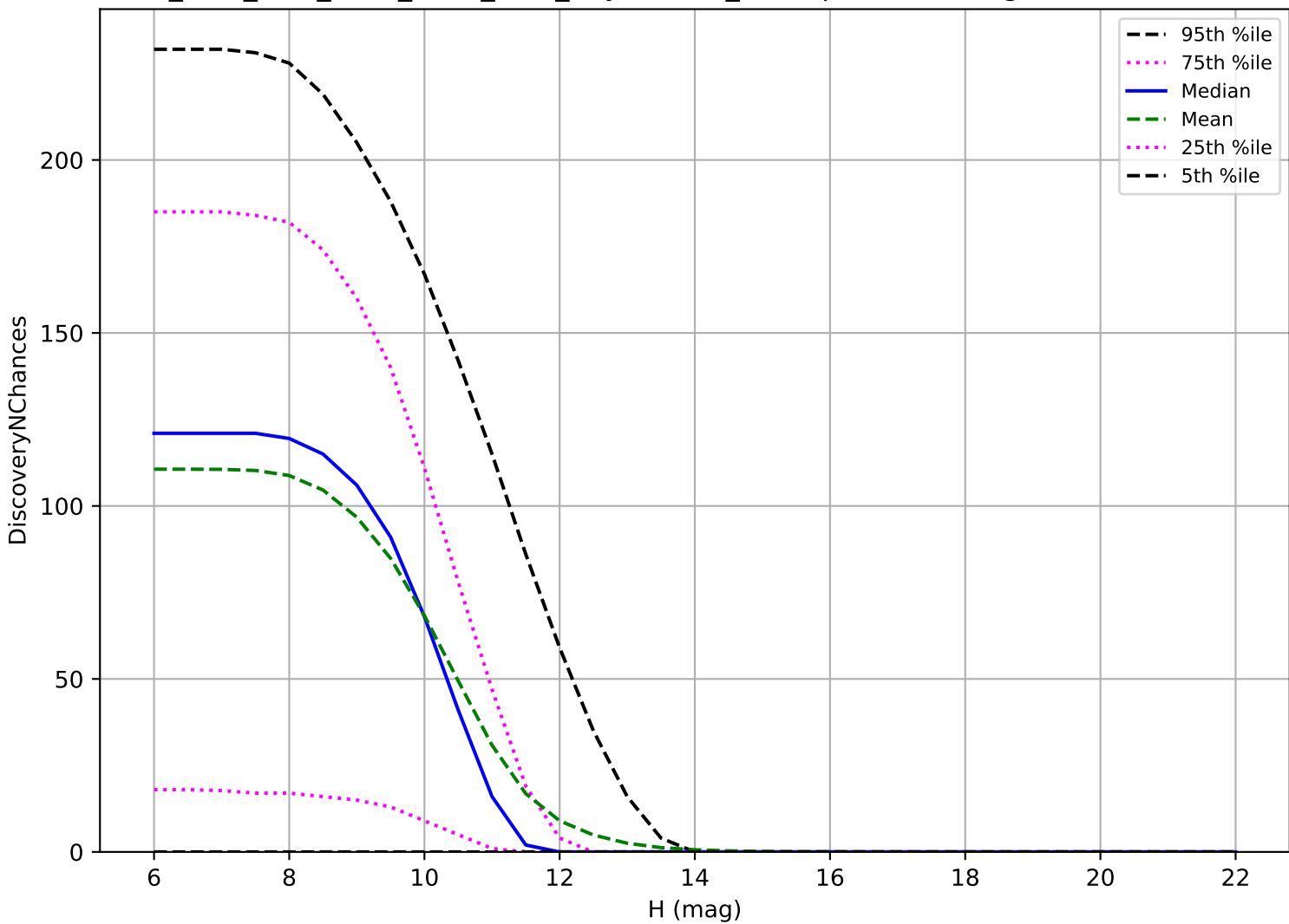
ddf_acor_sf10_lsf15_lsr10_v3.4_10yrs: OCC_r20 3 pairs in 15 nights detection loss
