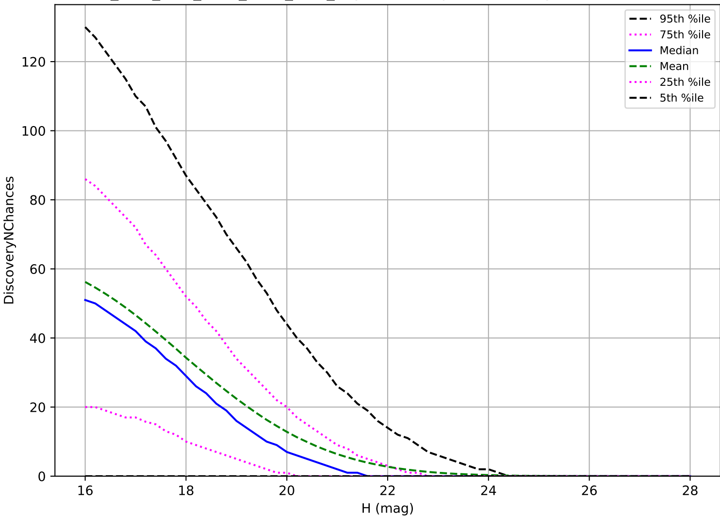
ddf_acor_sf10_lsf15_lsr10_v3.4_10yrs: NEO 3 pairs in 15 nights detection loss
