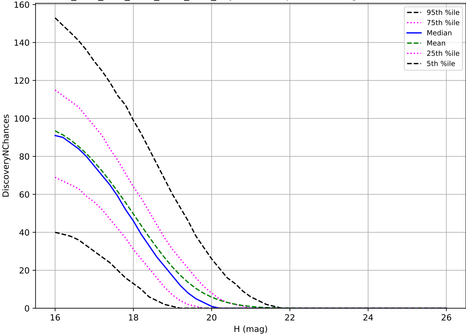
ddf_acor_sf10_lsf15_lsr10_v3.4_10yrs: MBA 3 pairs in 15 nights detection loss
