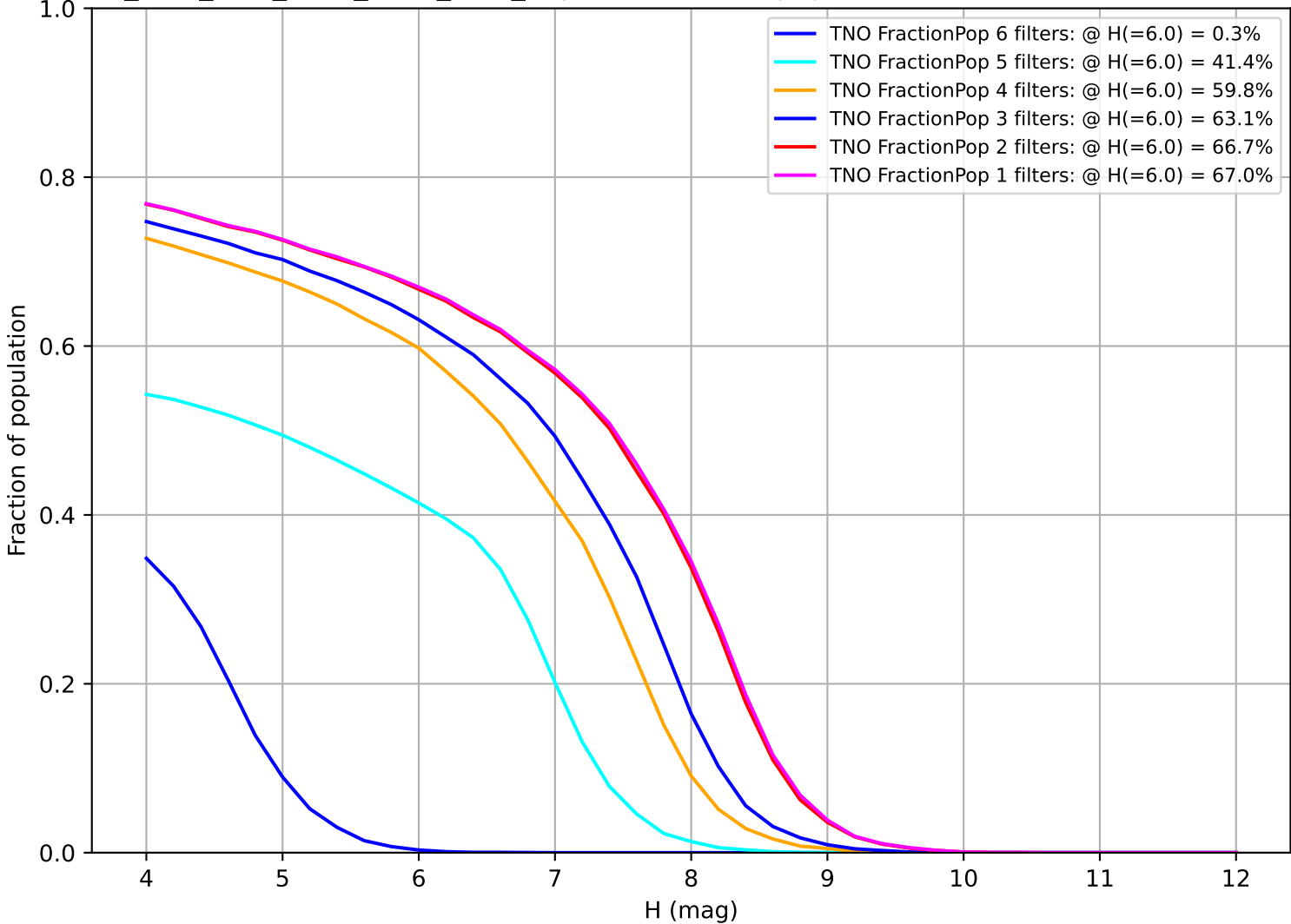
ddf_acor_sf10_lsf15_lsr10_v3.4_10yrs: Fraction of population with colors in X filters TNO
