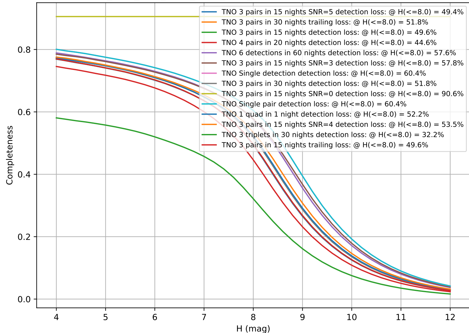
ddf_acor_sf10_lsf15_lsr10_v3.4_10yrs: CumulativeCompleteness
