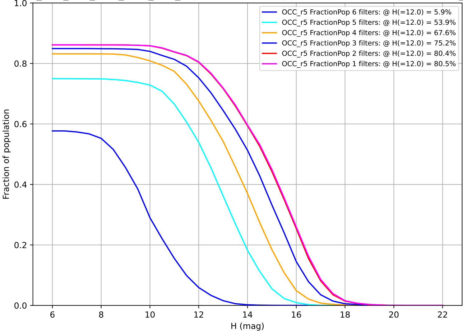
ddf_acor_sf10_lsf15_lsr10_v3.4_10yrs: Fraction of population with colors in X filters OCC_r5
