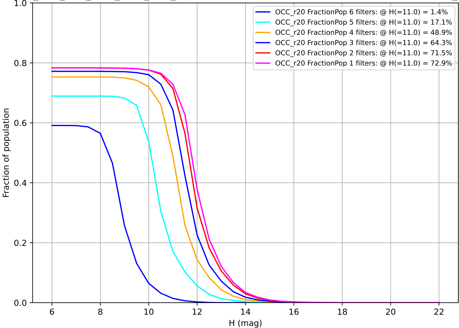
ddf_acor_sf10_lsf15_lsr10_v3.4_10yrs: Fraction of population with colors in X filters OCC_r20
