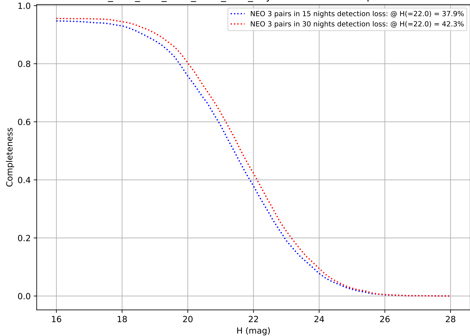
ddf_acor_sf10_lsf15_lsr10_v3.4_10yrs: DifferentialCompleteness
