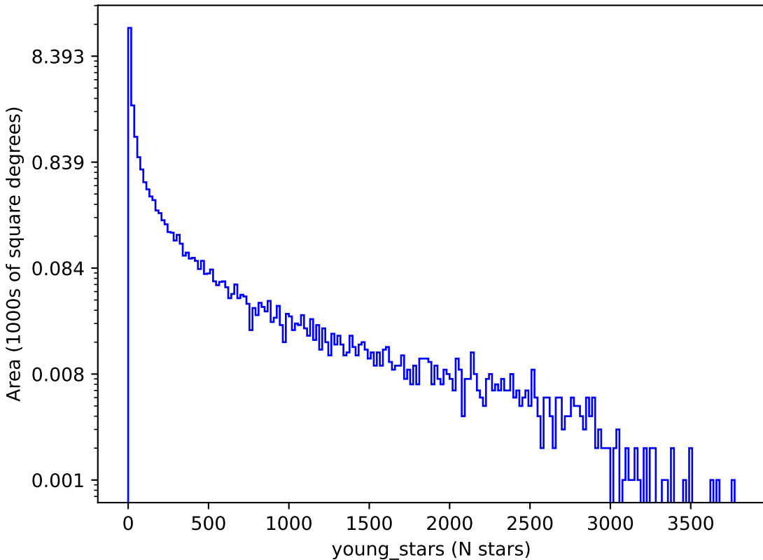
ddf_acor_sf10_lsf15_lsr10_v3.4_10yrs : young_stars
