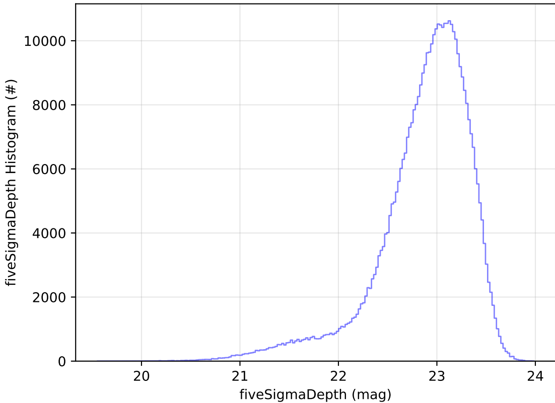
ddf_acor_sf10_lsf15_lsr10_v3.4_10yrs z: fiveSigmaDepth Histogram
