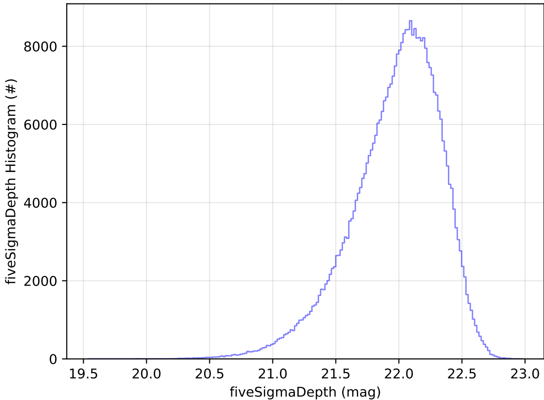
ddf_acor_sf10_lsf15_lsr10_v3.4_10yrs y: fiveSigmaDepth Histogram
