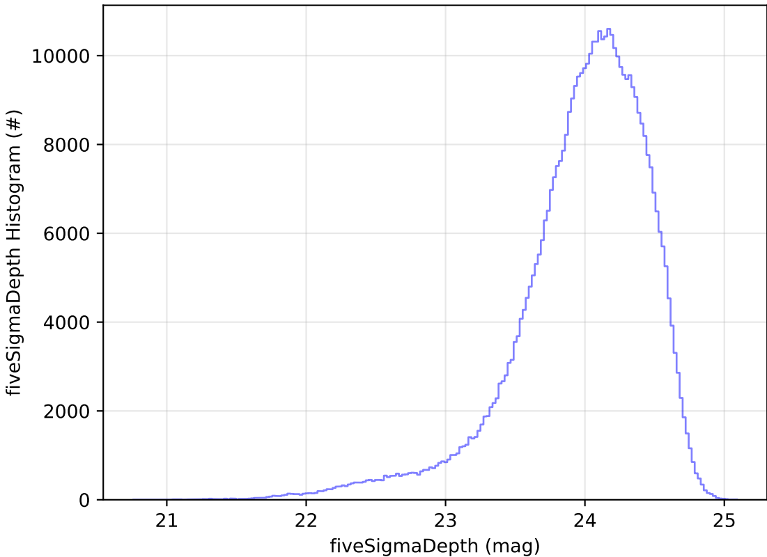
ddf_acor_sf10_lsf15_lsr10_v3.4_10yrs r: fiveSigmaDepth Histogram
