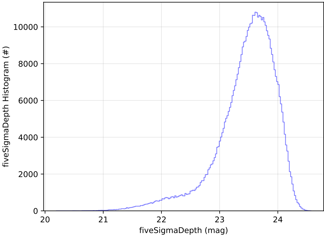
ddf_acor_sf10_lsf15_lsr10_v3.4_10yrs i: fiveSigmaDepth Histogram
