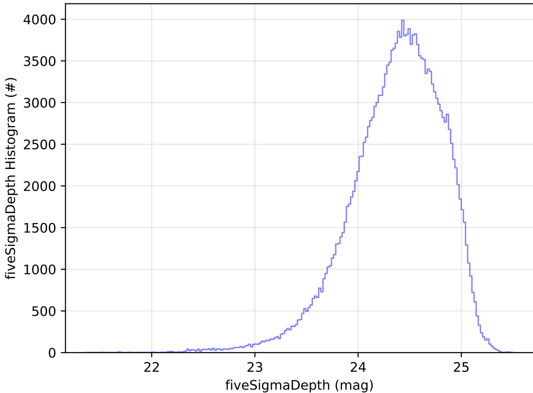
ddf_acor_sf10_lsf15_lsr10_v3.4_10yrs g: fiveSigmaDepth Histogram
