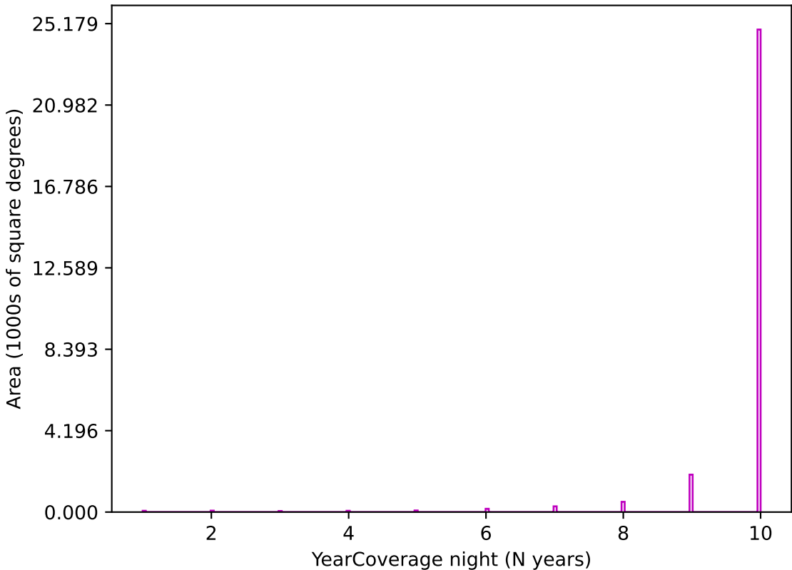
ddf_acor_sf10_lsf15_lsr10_v3.4_10yrs z band: YearCoverage night
