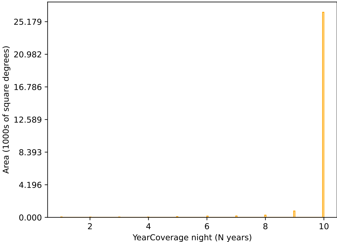
ddf_acor_sf10_lsf15_lsr10_v3.4_10yrs r band: YearCoverage night
