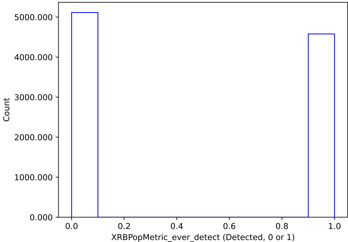
ddf_acor_sf10_lsf15_lsr10_v3.4_10yrs : XRBPpopMetric_ever_detect
