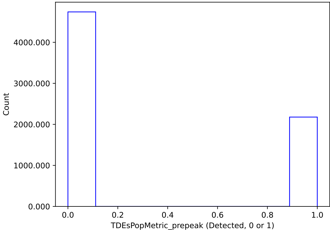
ddf_acor_sf10_lsf15_lsr10_v3.4_10yrs : TDEsPopMetric_prepeak
