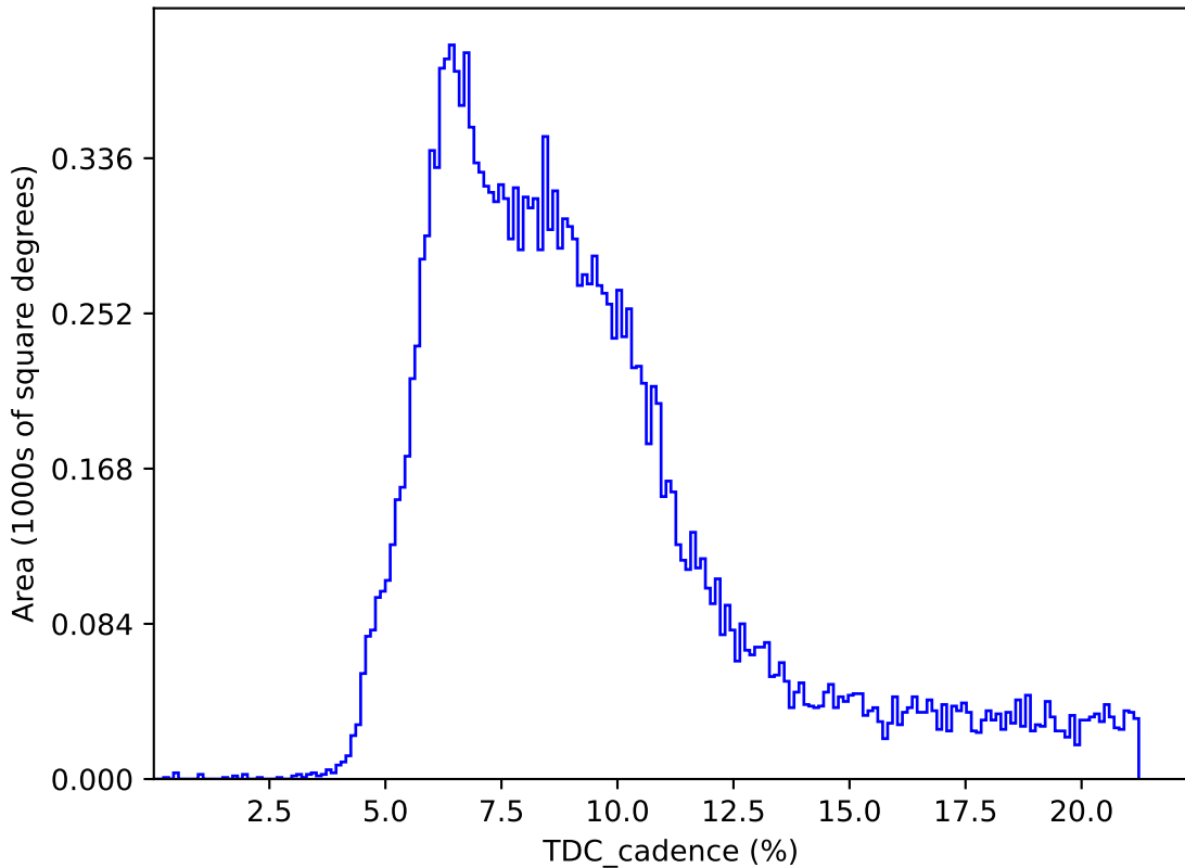
ddf_acor_sf10_ls15_lsr10_v3.4_10yrs : TDC_cadence
