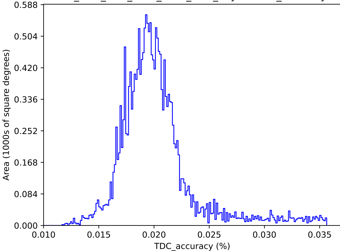
ddf_acor_sf10_lsf15_lsr10_v3.4_10yrs : TDC_accuracy
