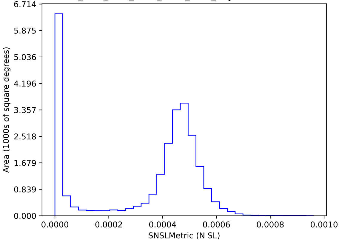
ddf_acor_sf10_lsf15_lsr10_v3.4_10yrs : SNSLMetric
