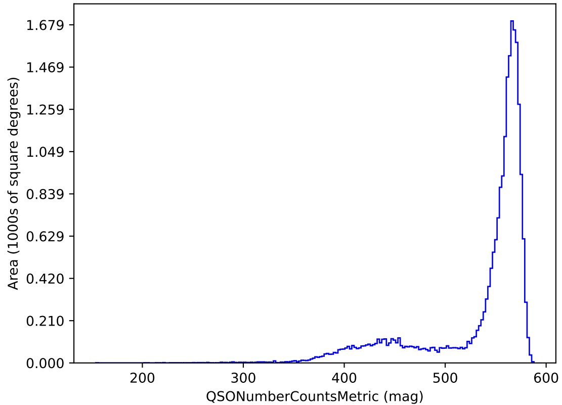
ddf_acor_sf10_lsf15_lsr10_v3.4_10yrs y band and non-DD: QSONumberCountsMetric
