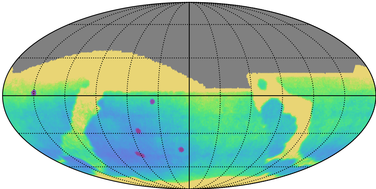
ddf_acor_sf10_lsf15_lsr10_v3.4_10yrs : Parallax Uncert @ 24.0
