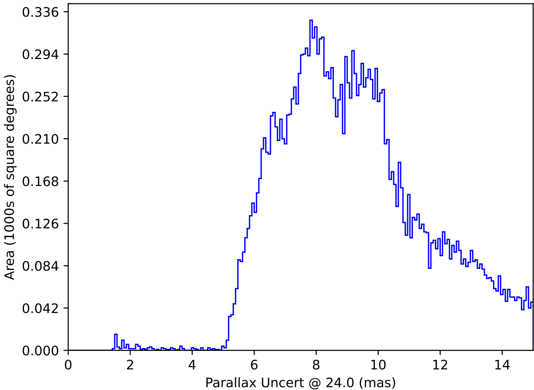
ddf_acor_sf10_lsf15_lsr10_v3.4_10yrs : Parallax Uncert @ 24.0
