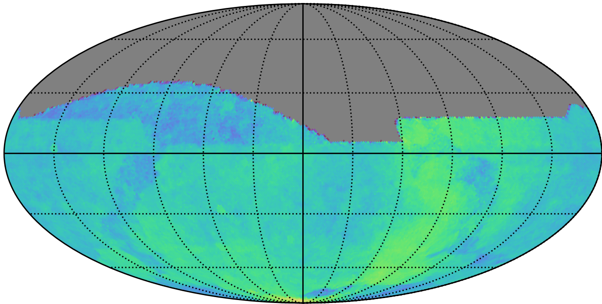
ddf_acor_sf10_lsf15_lsr10_v3.4_10yrs : Parallax Coverage @ 24.0
