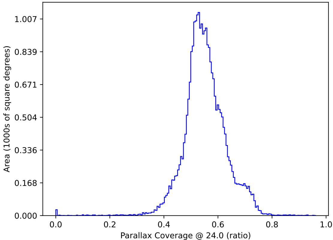
ddf_acor_sf10_lsf15_lsr10_v3.4_10yrs : Parallax Coverage @ 24.0
