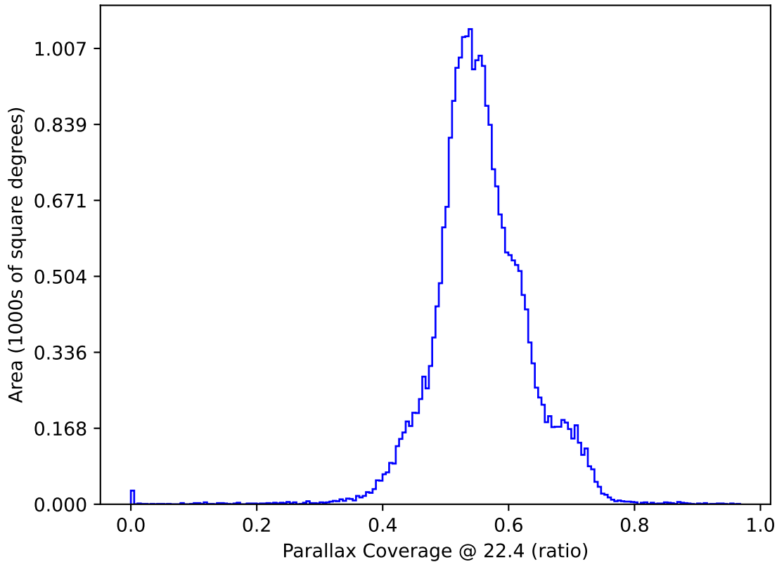
ddf_acor_sf10_lsf15_lsr10_v3.4_10yrs : Parallax Coverage @ 22.4
