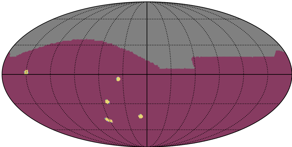
ddf_acor_sf10_lsf15_lsr10_v3.4_10yrs : NumberOfQuickRevisits
