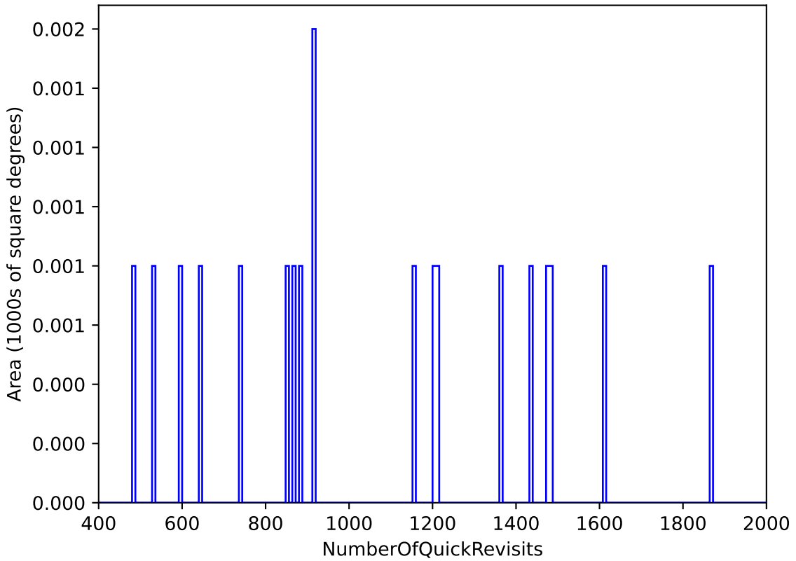
ddf_acor_sf10_lsf15_lsr10_v3.4_10yrs : NumberOfQuickRevisits
