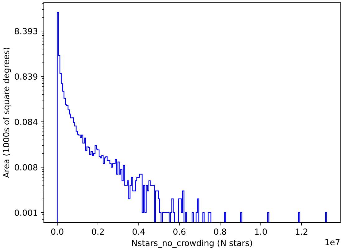
ddf_acor_sf10_ls15_lsr10_v3.4_10yrs g: Nstars_no_crowding
