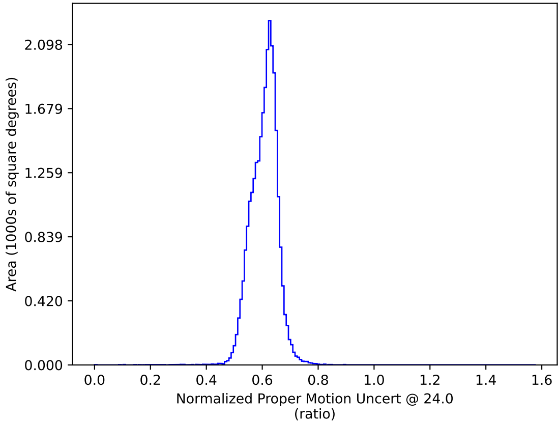
ddf_acor_sf10_lsf15_lsr10_v3.4_10yrs : Normalized Proper Motion Uncert @ 24.0
