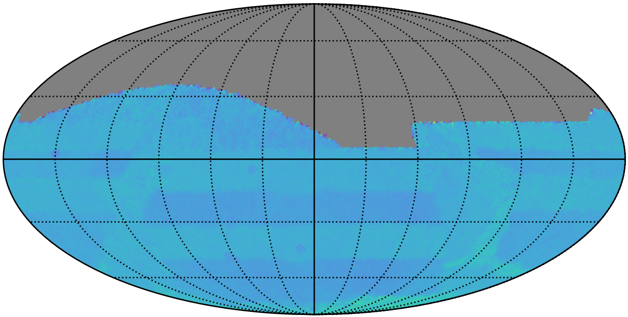
ddf_acor_sf10_lsf15_lsr10_v3.4_10yrs : Normalized Proper Motion Uncert @ 20.5
