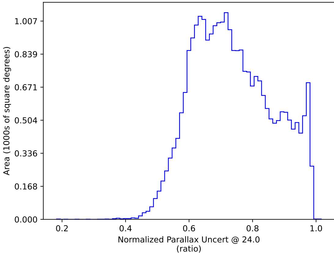
ddf_acor_sf10_lsf15_lsr10_v3.4_10yrs : Normalized Parallax Uncert @ 24.0
